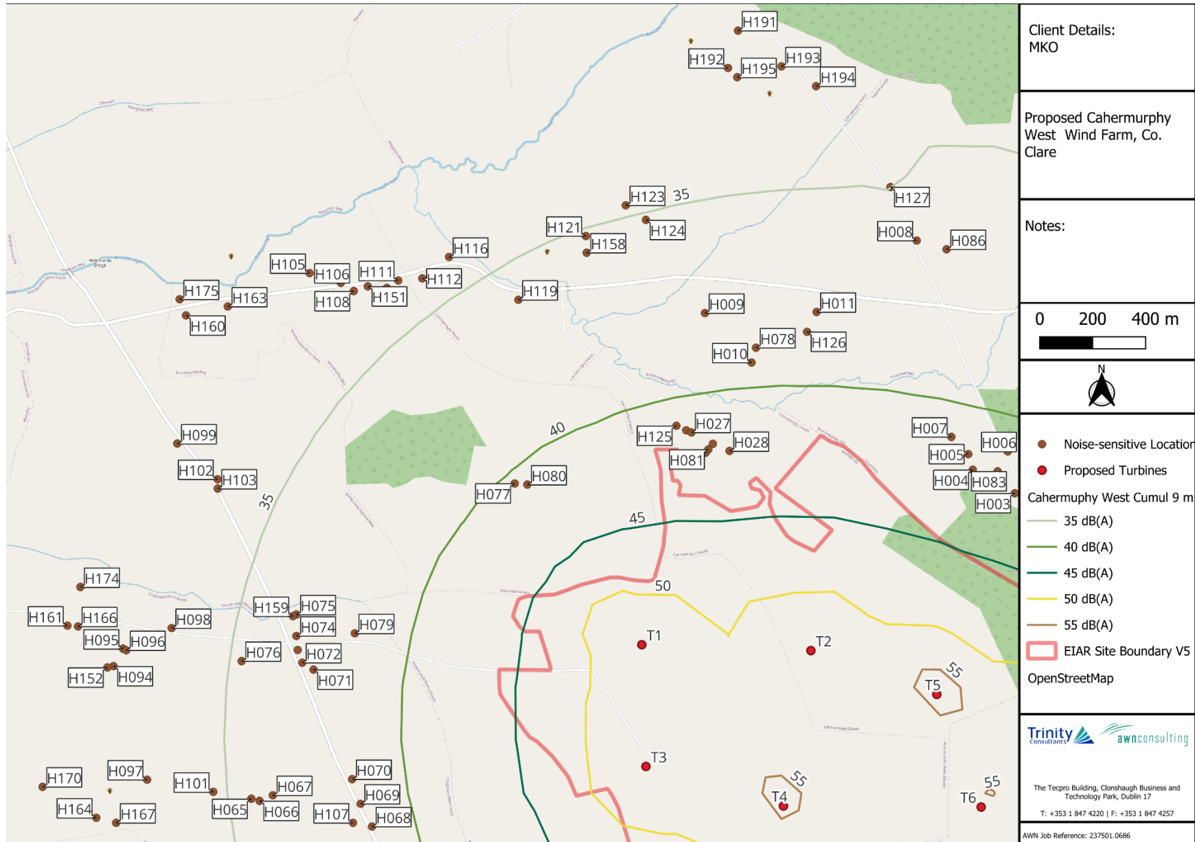
Figure 12-8-2. Predicted Cumulative Noise Contours Detail 1 of 4
