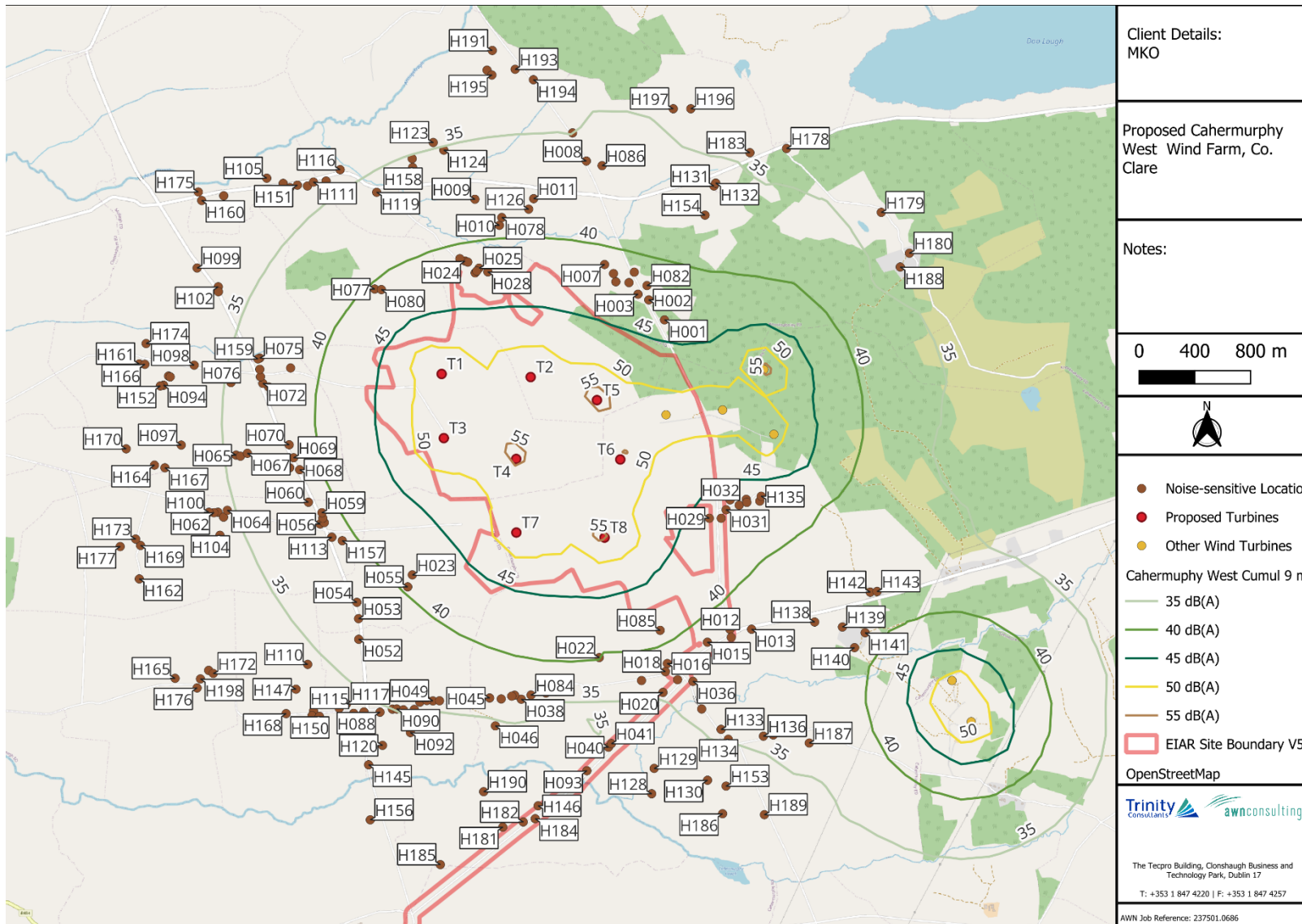
Figure 12-8-1. Predicted Cumulative Noise Contours Overall
