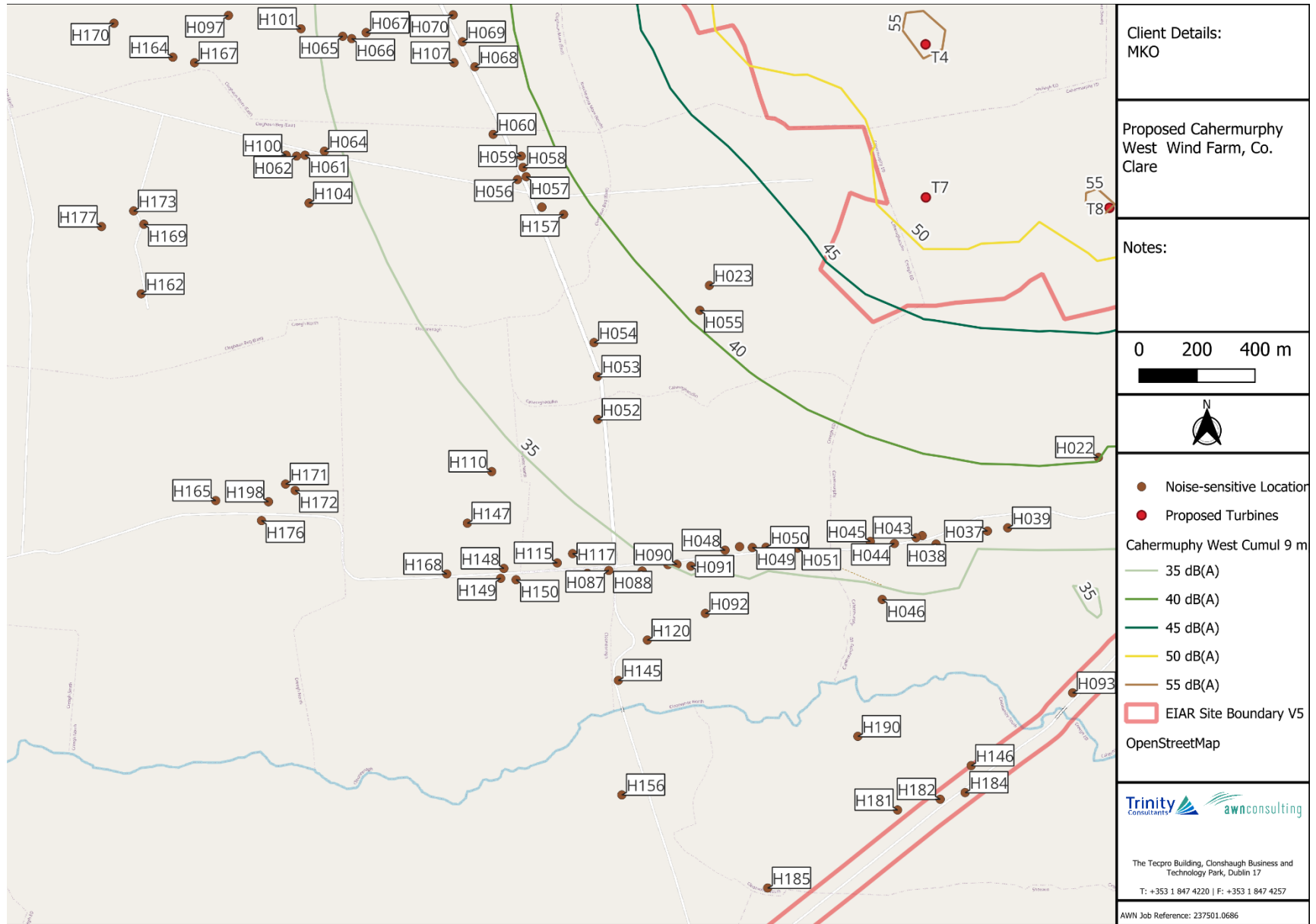
Figure 12-8-5. Predicted Cumulative Noise Contours Detail 4 of 4
