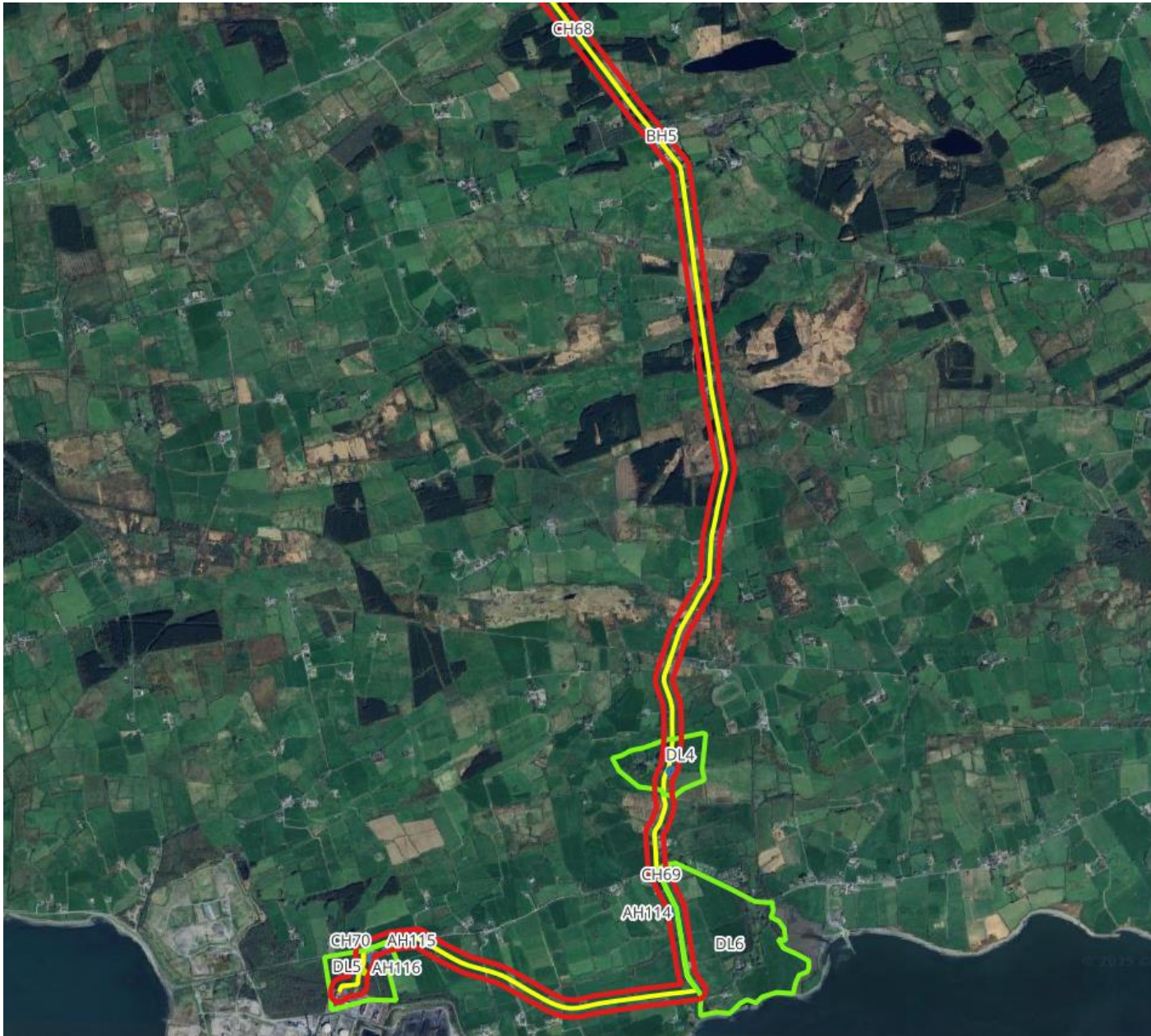
Figure 13-4 Southern section of GCR, showing archaeological, architectural and cultural heritage sites
